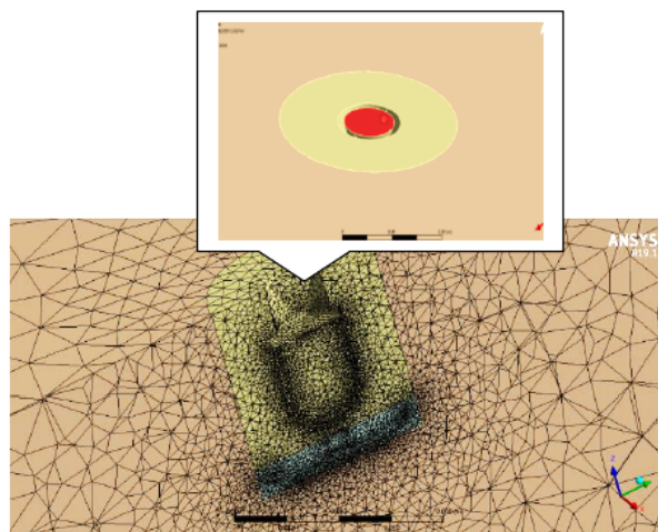
Fig. 2. Selected surface as water inlet
