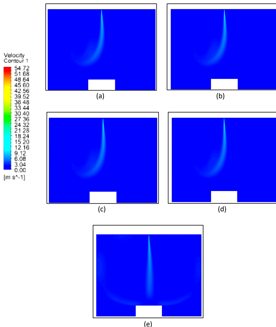
Fig. 5. Distribution of water discharged from fire sprinkler at different operating pressure (a) Model A (b) Model B (c) Model C (d) Model D (e) Model E
