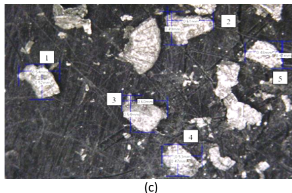
Fig. 8. Microstructure after milling (a) 2 hours (b) 4 hours (c) 6 hours
