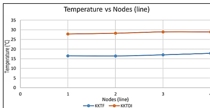
Fig. 8. Experimental temperature results
