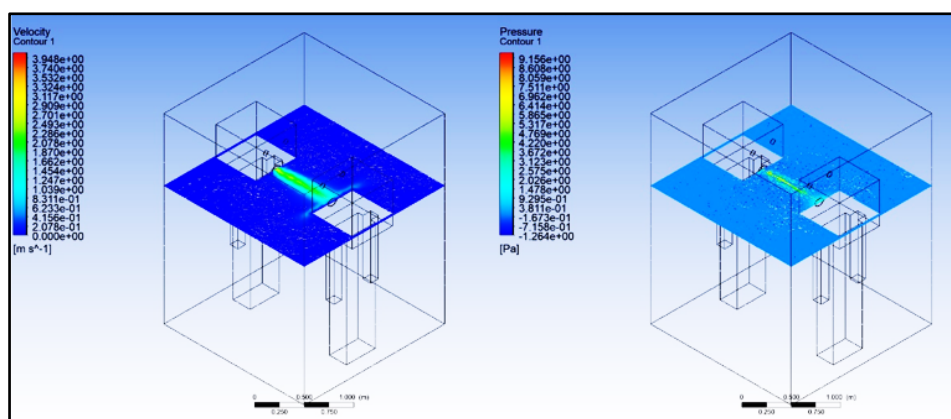
Fig. 4. 2-person with inlet velocity 3.19 m/s
