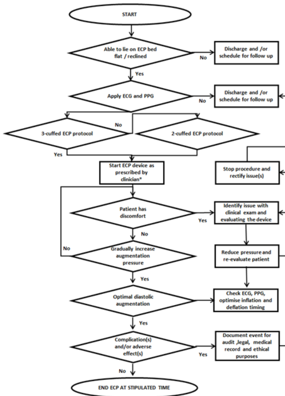
Fig. 9. The proposed workflow during the ECP session. * Indicates that the clinician would determine the number of cuffs to be used, the trigger ratio, and cuff pressures for the session
