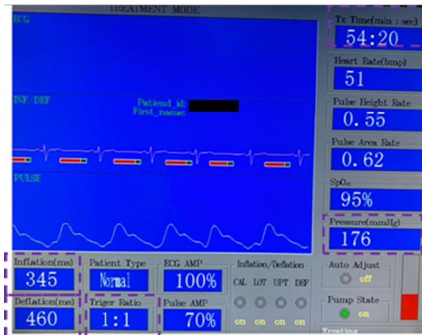
Fig. 7. Example of an ECP system display. The purple dash boxes are parameters that may be adjusted during the ECP treatment
