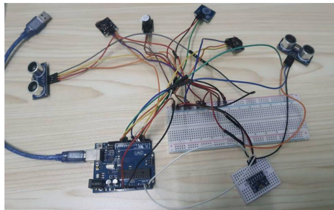
Fig. 7. Prototype of the StepSafe Cane
