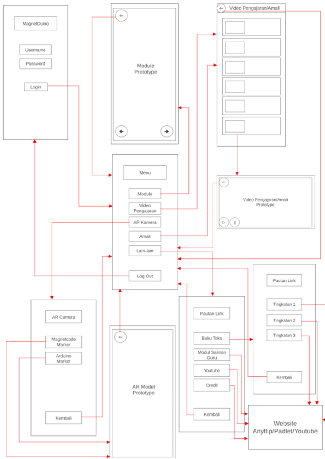
Fig. 5. Application wireframe
