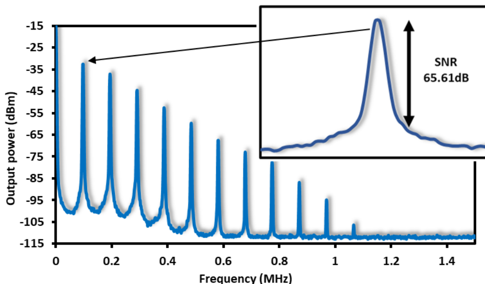
Fig. 6. RF spectrum
